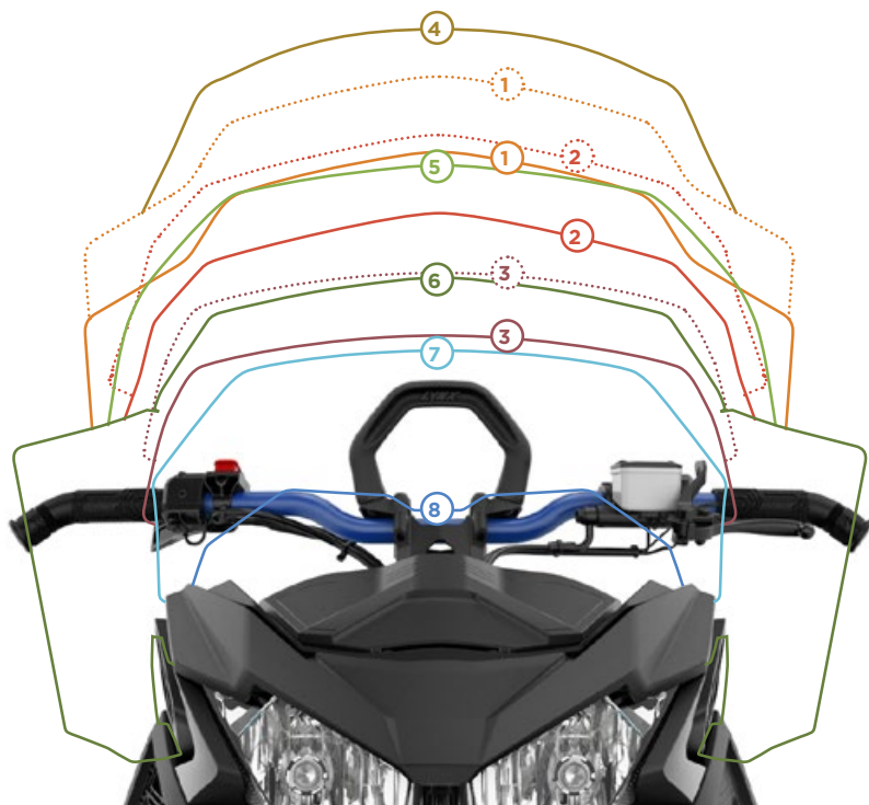
WINDSHIELD, LOW 860202262 36 cm high. Includes windshield support. RADIEN / RADIEN-X
